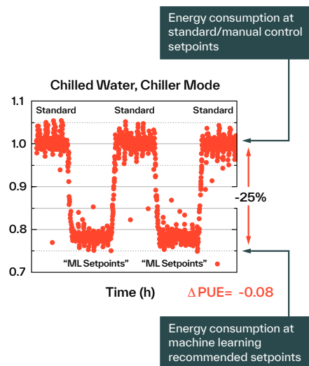
Figure 5: Normalized power-dissipation 1
